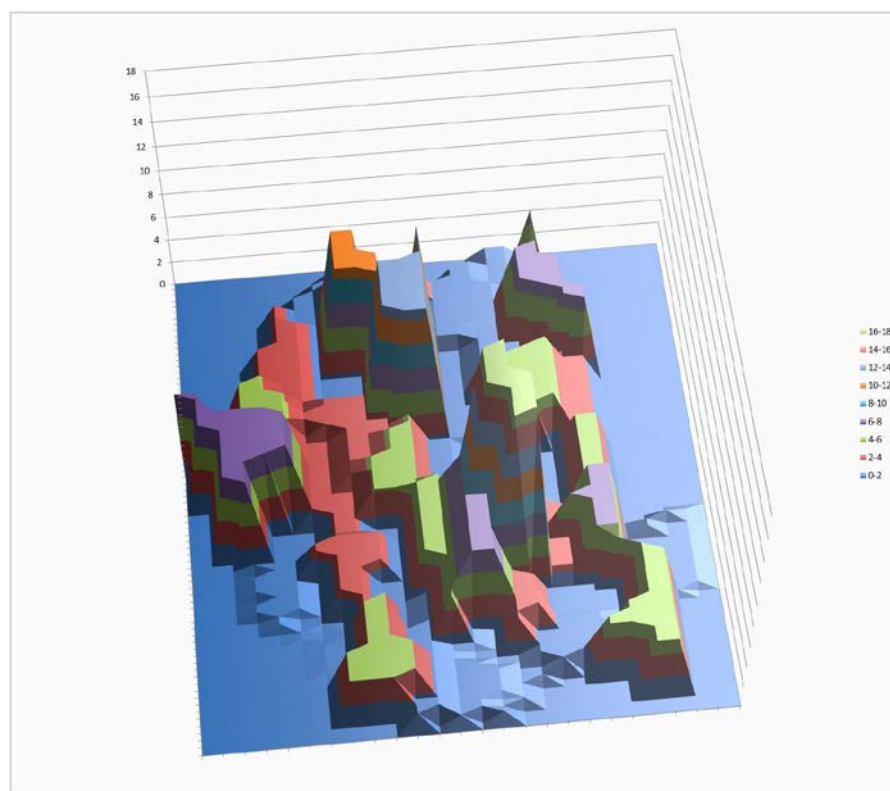
Figure 3 Romania gas grid CC and mechanical risk [probable deaths/1000 cap]
