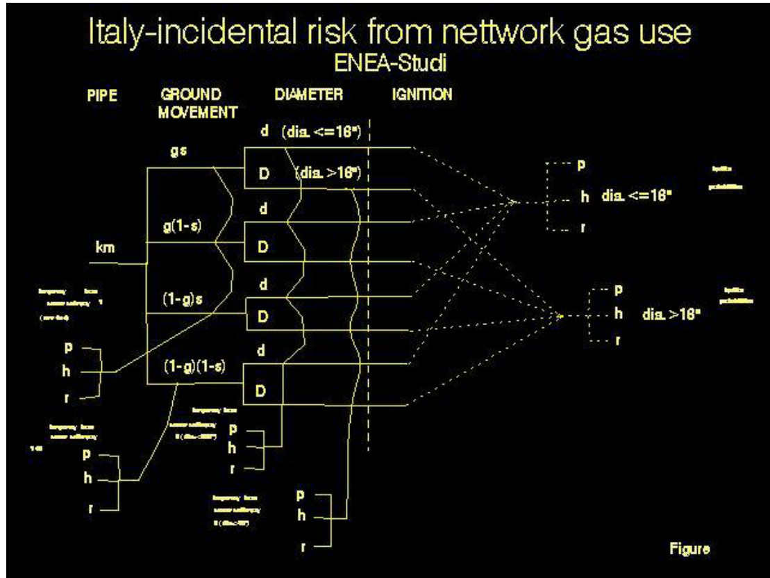
Figure 1. event tree for risk evaluation.
